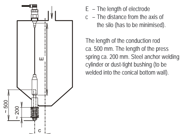
CLM-36_-31 Installation of rope electrode with anchor
