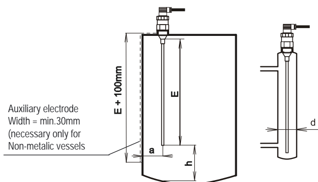
CLM-36_-10, 12 Installation in metallic or non-metallic vessels
