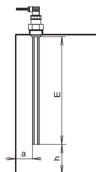
CLM-36_-40-G Non-metallic vessels and aggressive liquids
