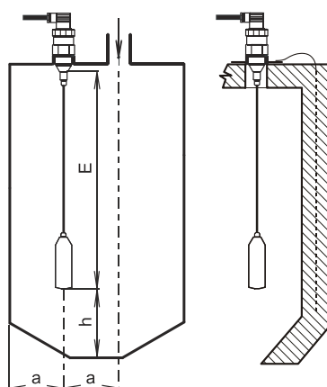
CLM-36_-30 Installation in containers and silos CLM-36_-32 Installation in deep vessels and sumps
