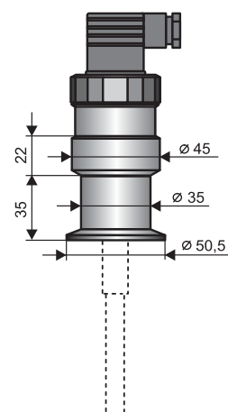
Housing with Tri-clamp coupling
