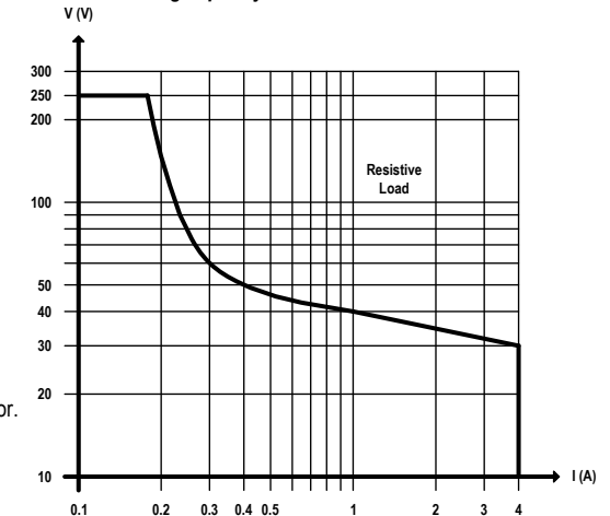
DC Load breaking capacity:
