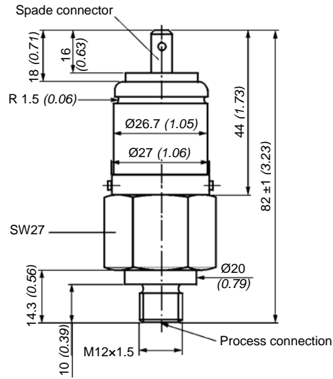
Fig. 8: Piston pressure switch type KD1-...-A1
