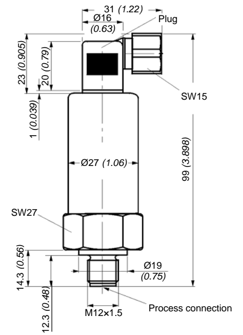
Fig. 10: Piston/diaphragm pressure switch type KLK/KLM-...-S1
