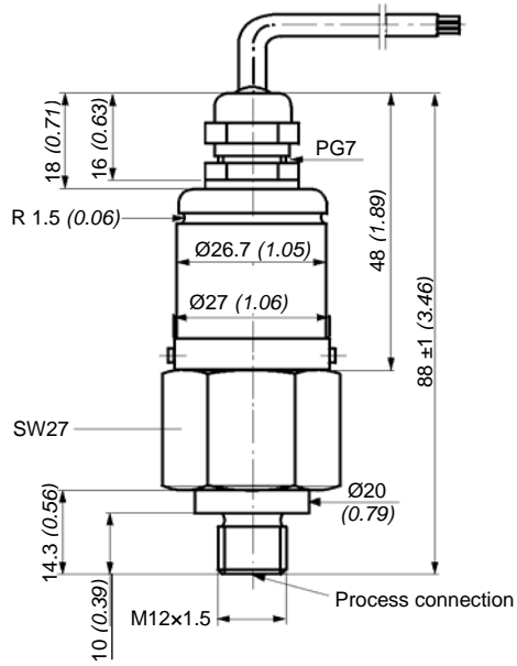
Fig. 7: Piston pressure switch type KD1-...-K2
