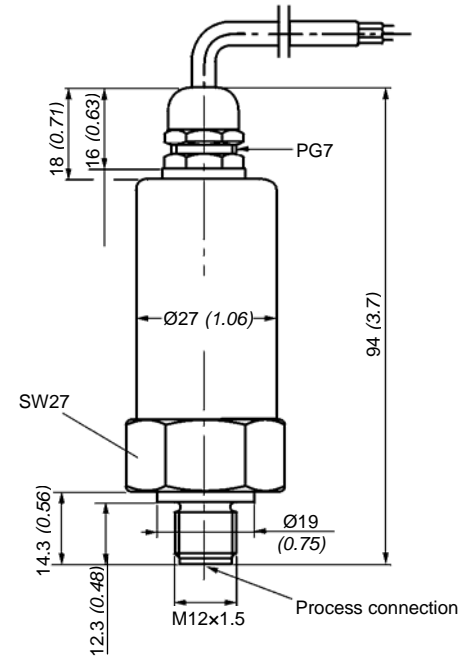
Fig. 9: Piston/diaphragm pressure switch type KLK/KLM-...-K2
